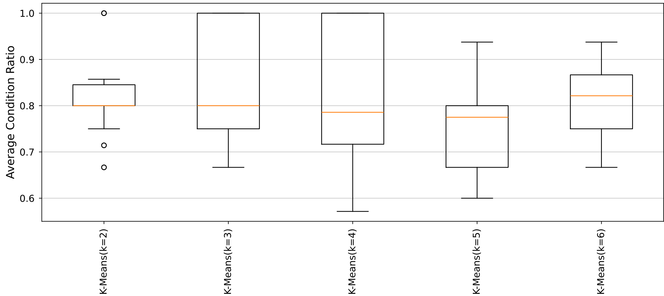
YARA Rules Average Condition Ratio Distribution (Cluster18_Size6 dataset)
